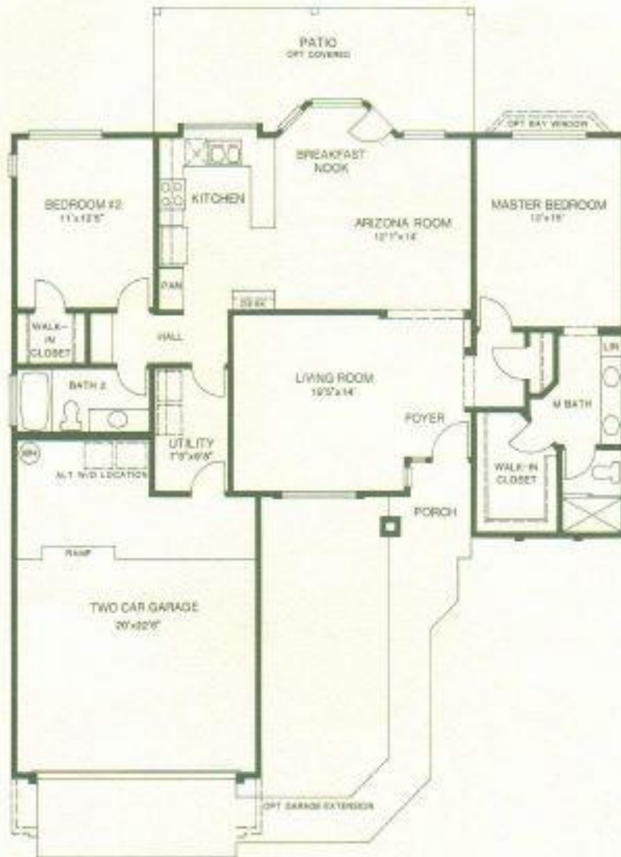
Plan 702 1430 Sq. Ft.
